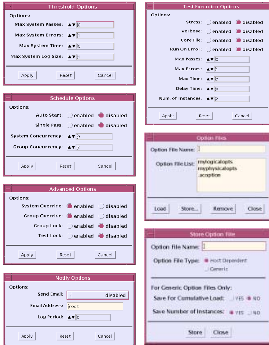
FIGURE 1-3 SunVTS CDE Option Menus
