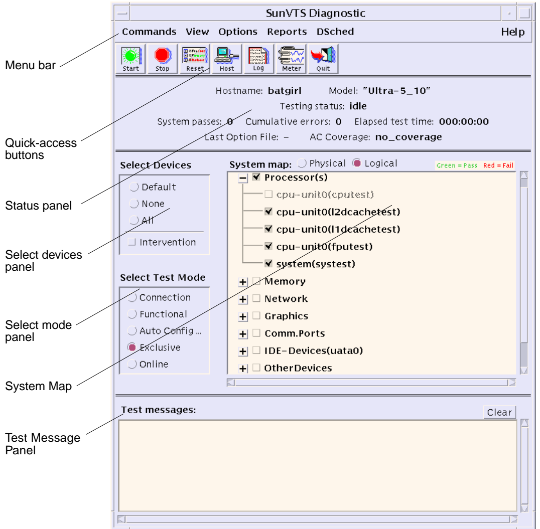
FIGURE 1-1 SunVTS CDE Main Window
